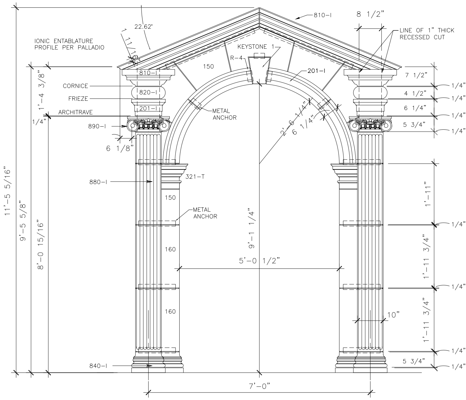
1 IONIC PILASTER WITH ARCH AND PEDIMENT
