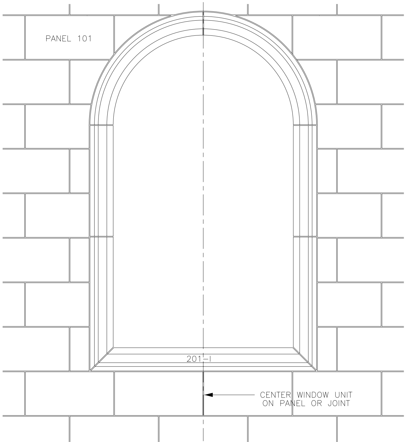
1 ARCHED WINDOW SURROUND WITH PROFILE 201-I
