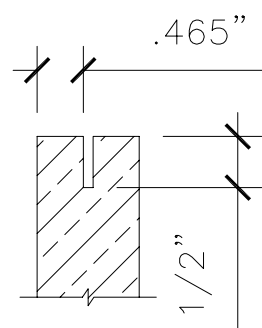
3 DETAIL – ANCHOR SLOT
