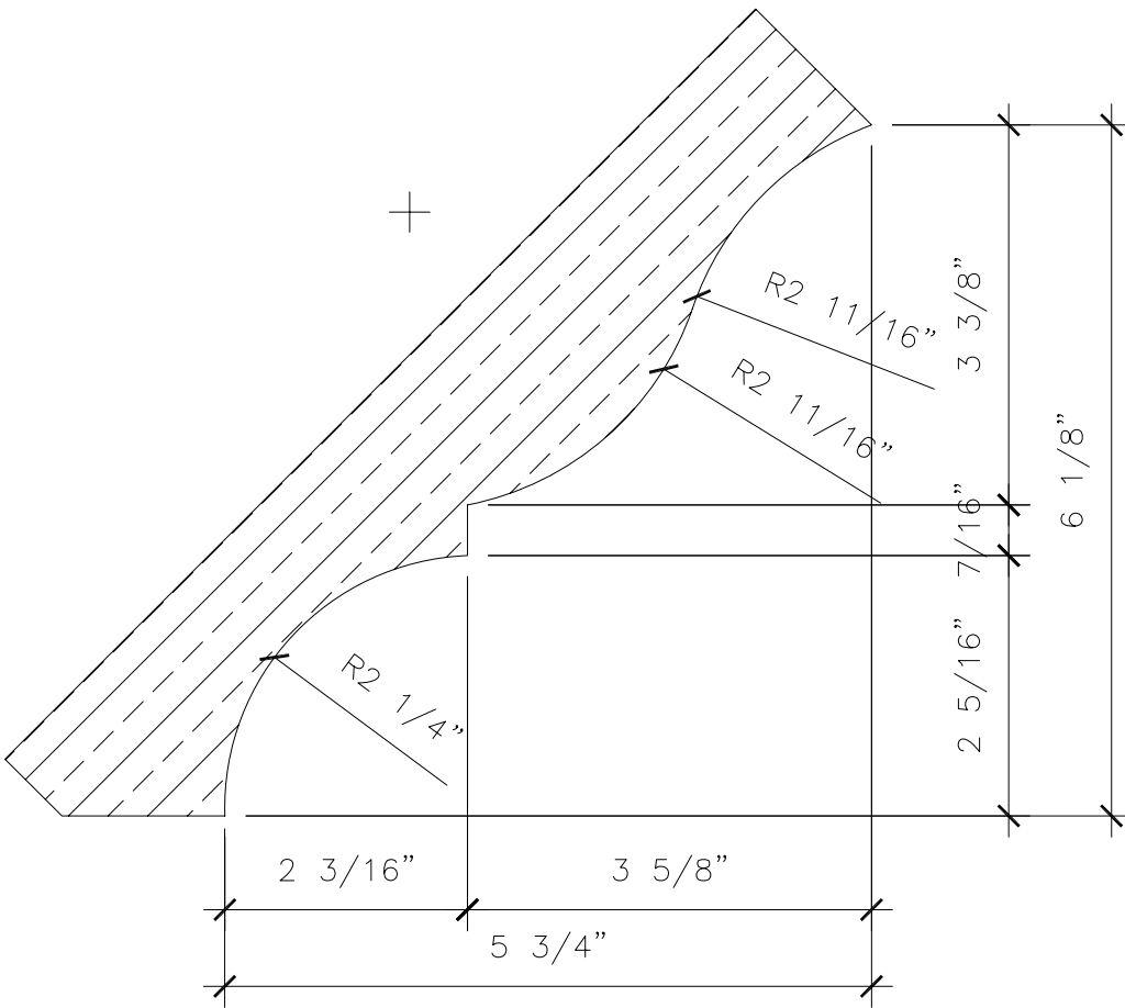
1 PROFILE 310-T
