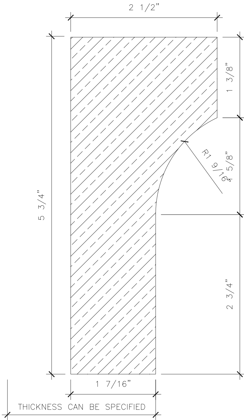
1 PROFILE 320-T
