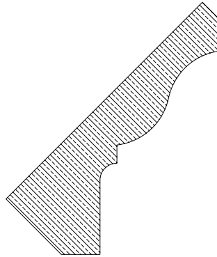
PROFILE 301-T 18 LBS. PER LINEAR FOOT DIAMOND TOOL MADE FOR THIS
