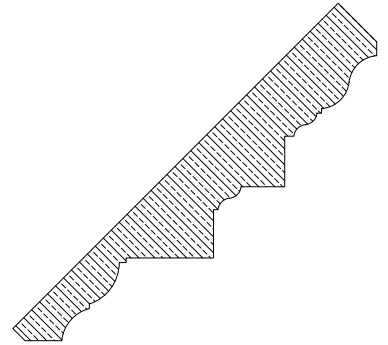
PROFILE 810-I 17 LBS. PER LINEAR FOOT
