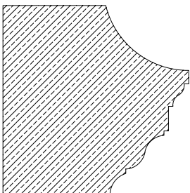
PROFILE 850-I 21 LBS. PER LINEAR FOOT
