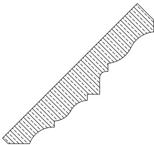
PROFILE 907-M 19 LBS. PER LINEAR FOOT DIAMOND TOOL MADE FOR THIS
