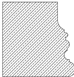
PROFILE 840-B BRICK COMPATIBLE 39 LBS. PER LINEAR FOOT DIAMOND TOOL MADE FOR THIS
