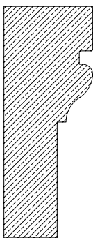
PROFILE 202-M 12 LBS. PER LINEAR FOOT
