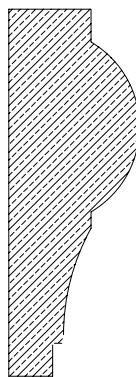
PROFILE 203-M 10 LBS. PER LINEAR FOOT DIAMOND TOOL MADE FOR THIS
