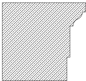
PROFILE 201-B BRICK COMPATIBLE 36 LBS. PER LINEAR FOOT DIAMOND TOOL MADE FOR THIS
