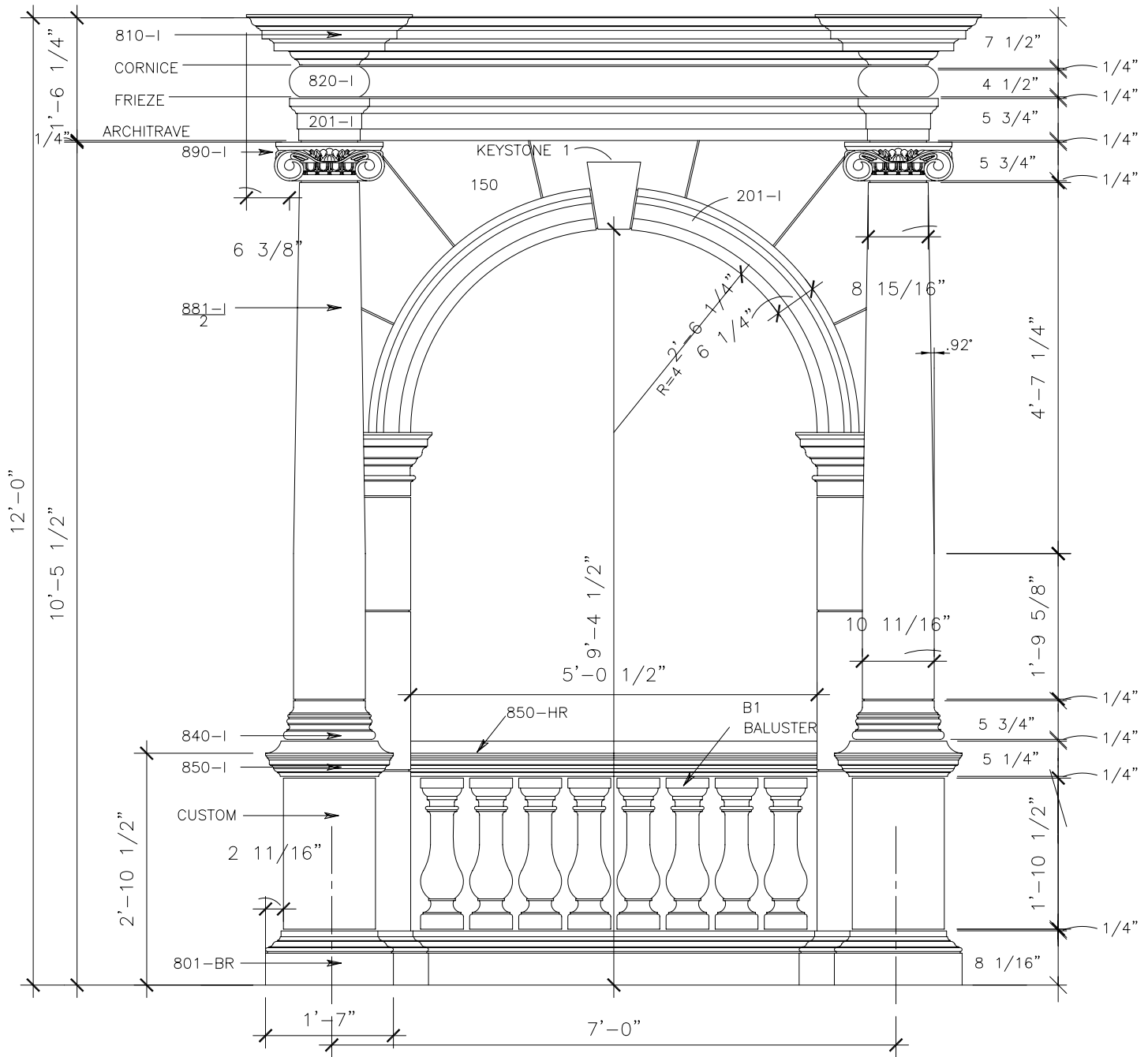
1 IONIC COLUMNS WITH BALUSTRADE AND ENTABLATURE OTHER BALUSTER SIZES AND TYPES ARE AVAILABLE
